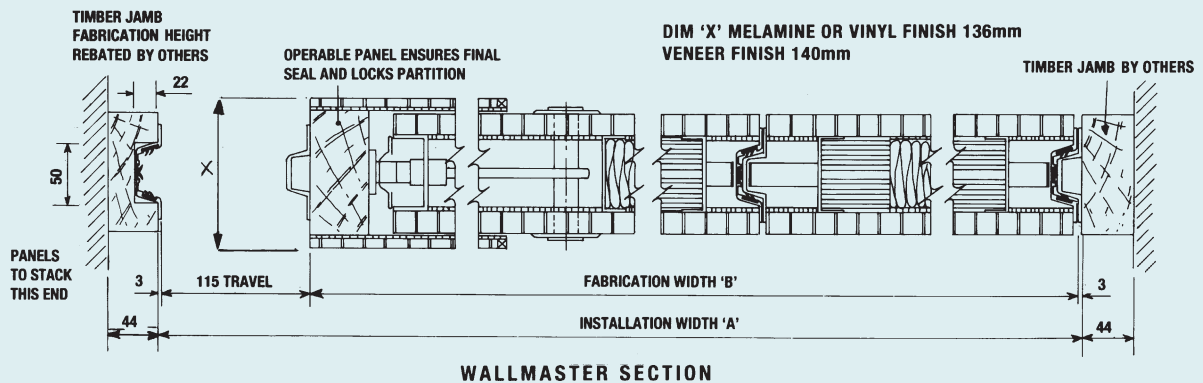
WALLMASTER SECTION
