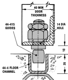
METAL DOORS ANY WIDTH
