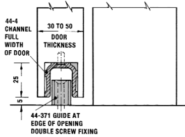
GUIDING FOR INTERIOR TIMBER DOOR UP TO 1500mm WIDE
