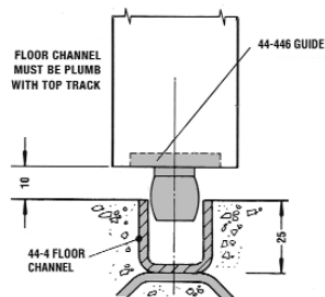
TIMBER DOORS OVER 1500MM WIDE
