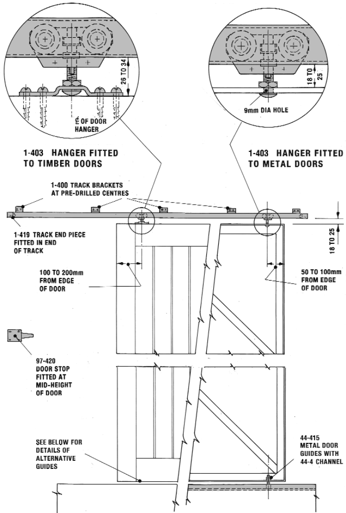
ELEVATION OF TIMBER AND METAL DOORS
