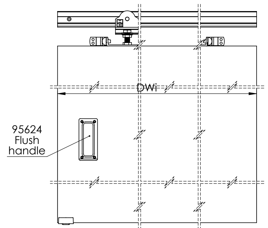
Front view Scale 1:5
