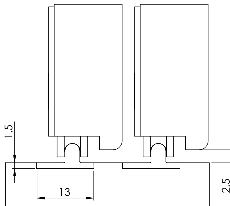
Front view With partly recessed track
