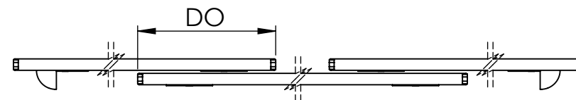
Top view Three doors on two tracks Scale 1:14
