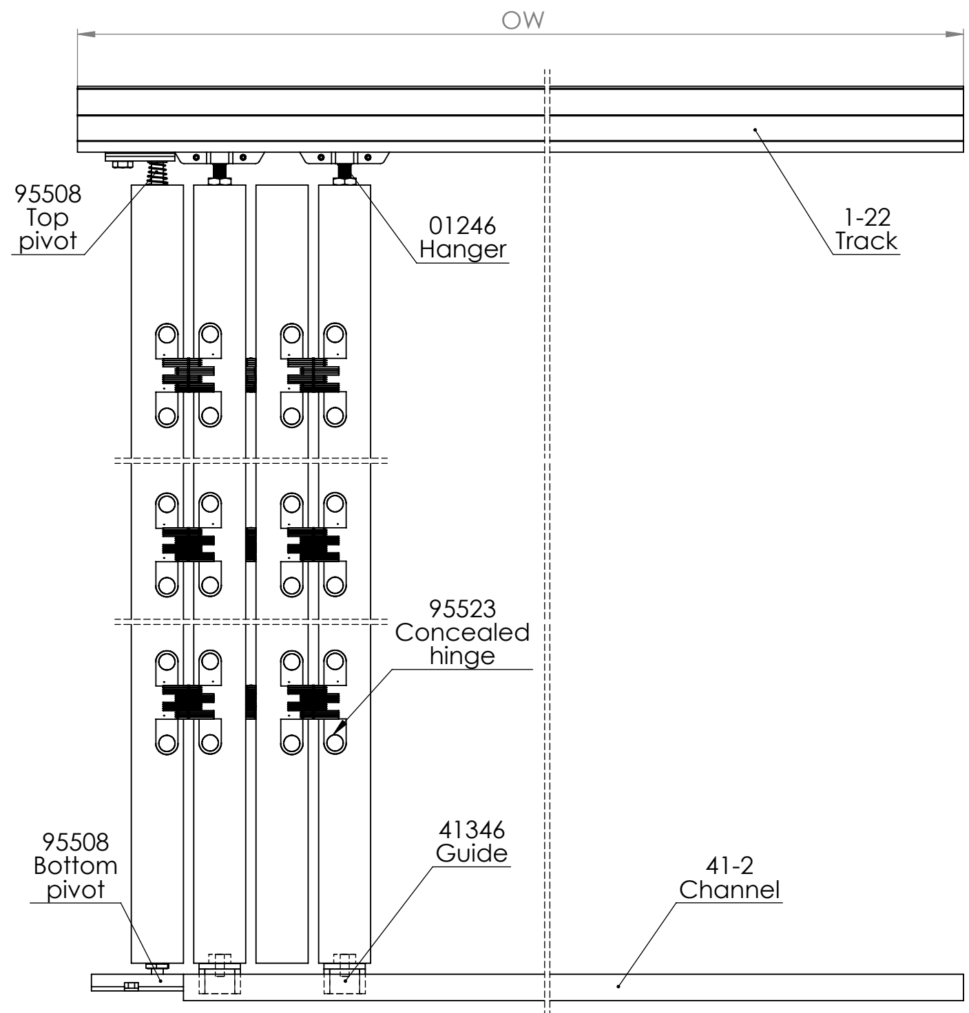
Front view with doors in fully closed position
