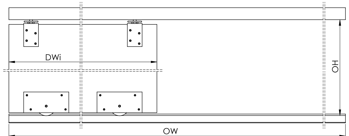
Front view With timber door Scale 1:6
