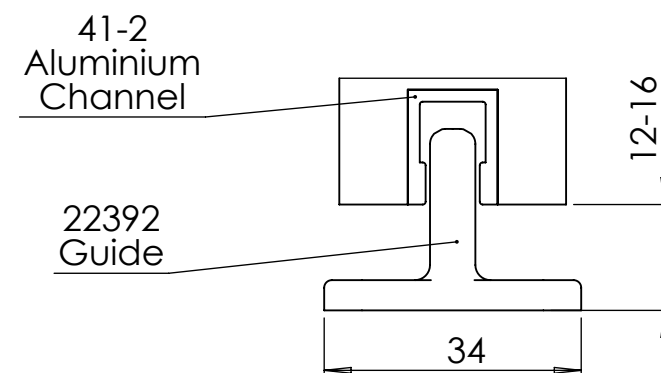
Side view Timber Door Alternative Bottom Guide
