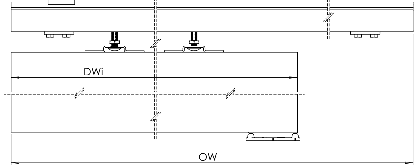
Front view With Timber Door Scale 1:3
