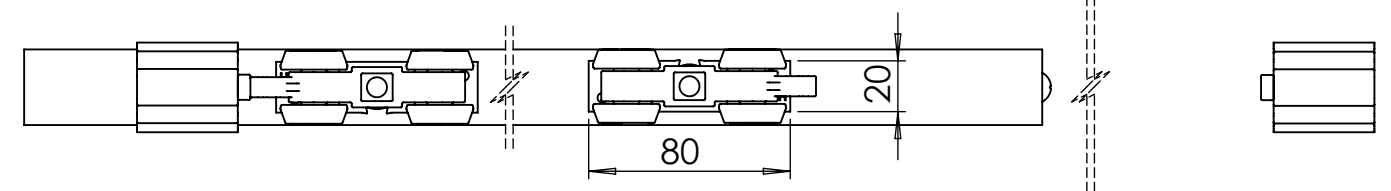
Front view With Timber Door Scale 1:3
