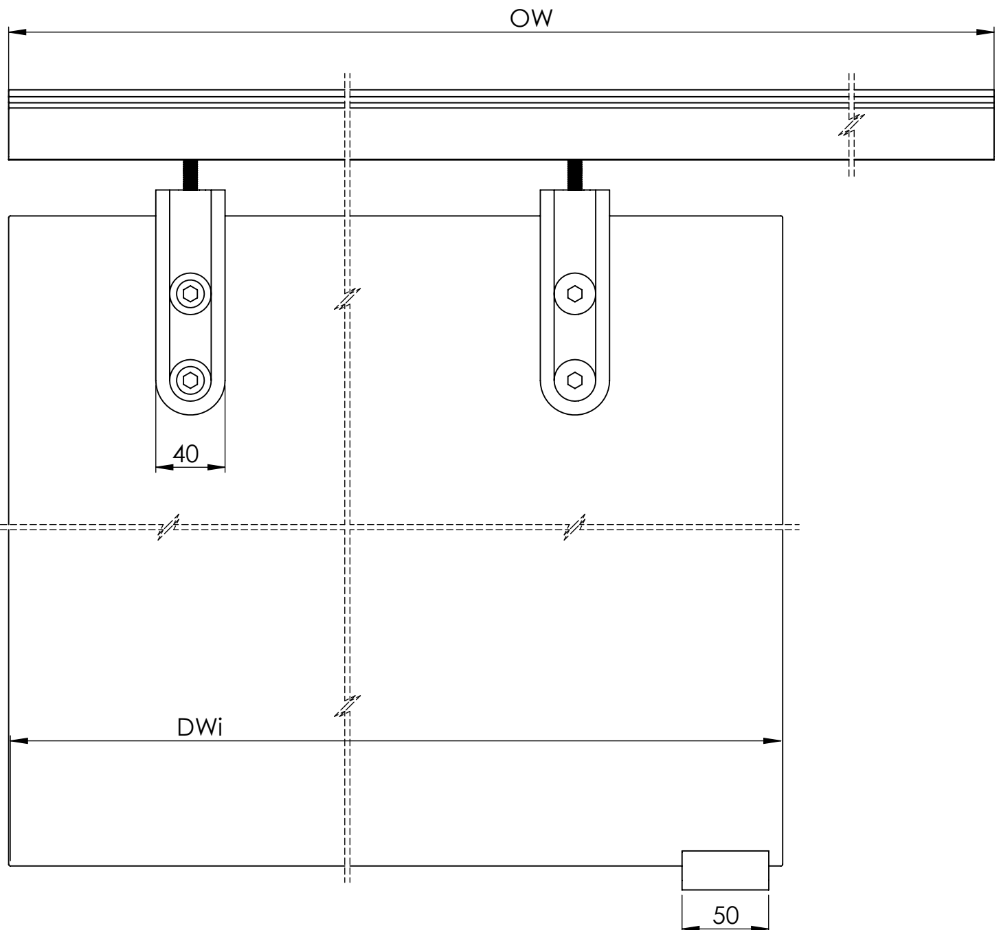
Front View Scale 1:5
