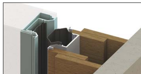
Door stile and telescopic jamb profiles
