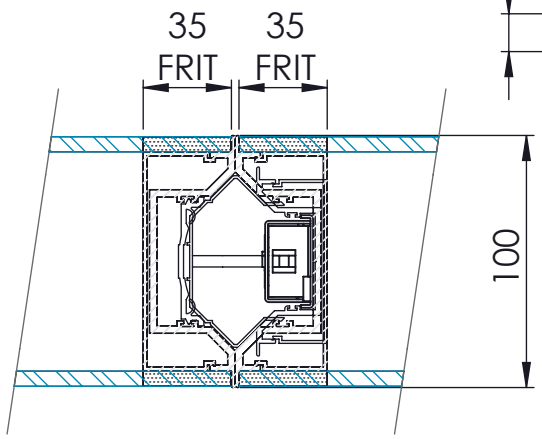
TYPE GS100 PANEL JOINT
