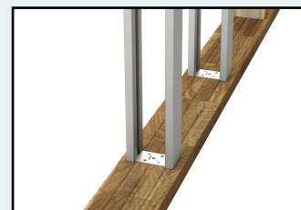
Self adjusting floor plates
