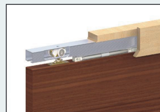
Track c/w hanger and integrated soft closer
