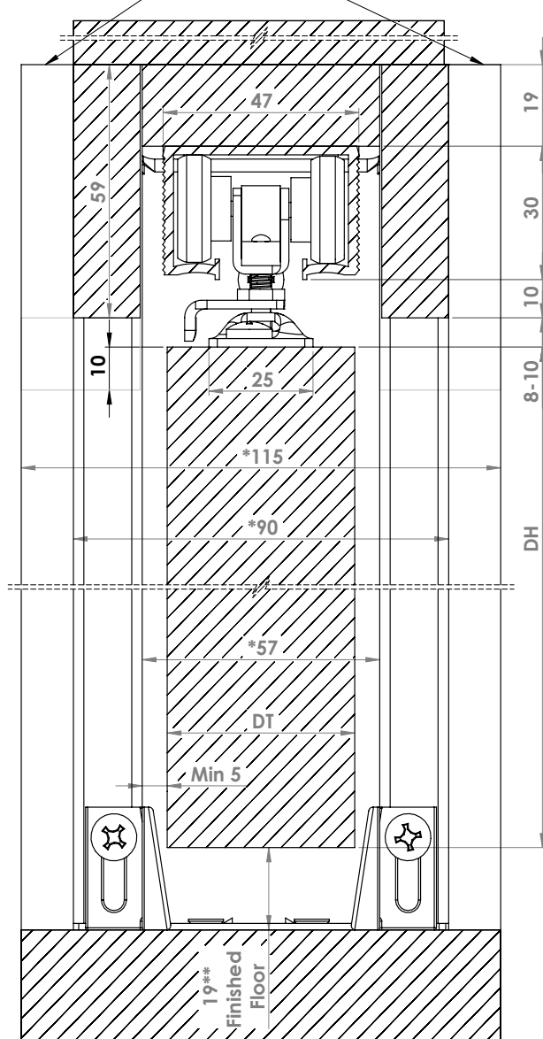
Side view with alternative bottom guide Scale 1:2
