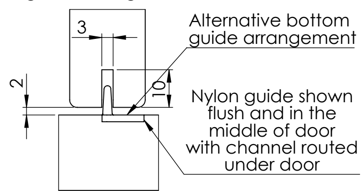
Side view with alternative guide arrangement
