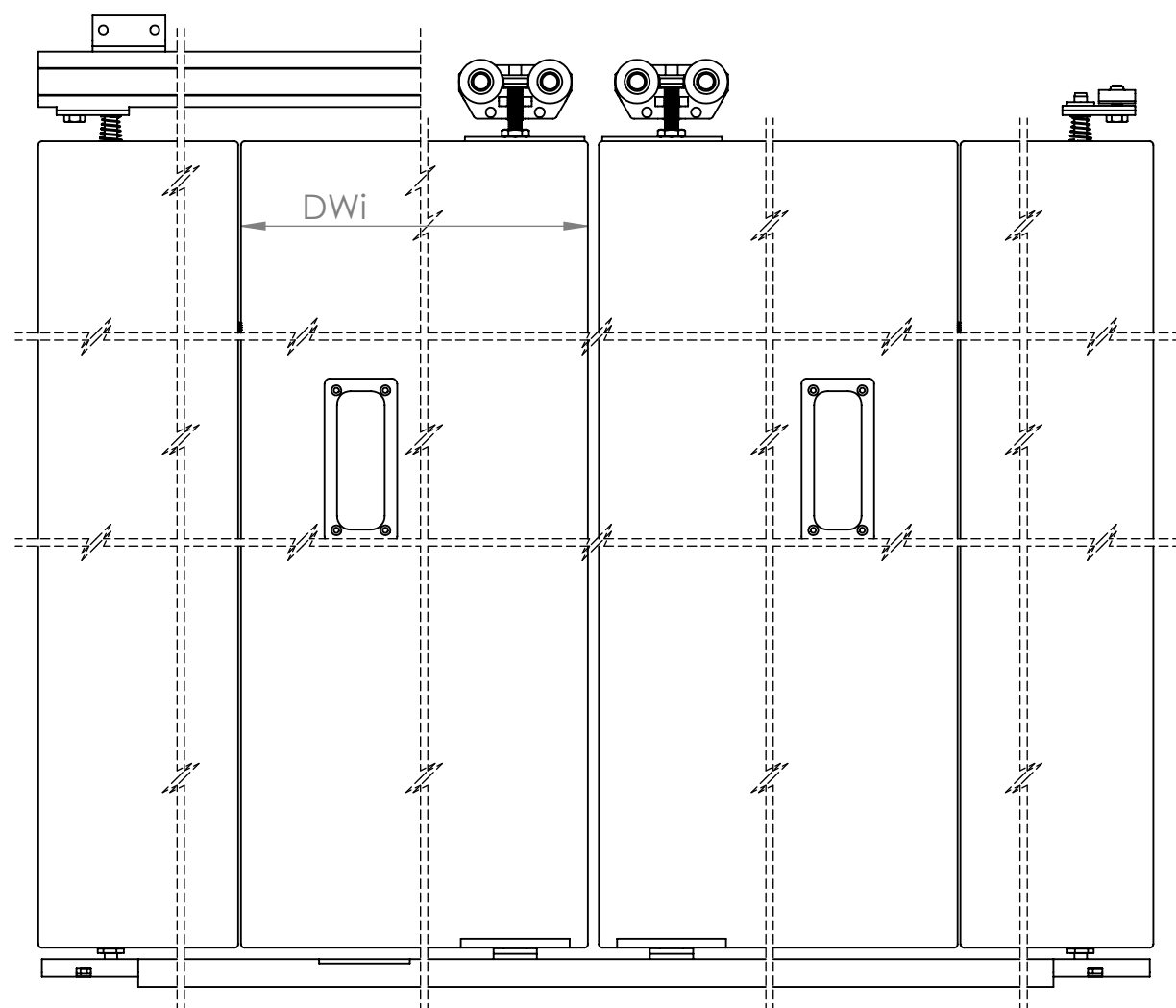
Front view Scale 1:4
