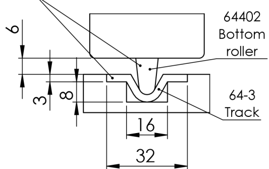
Alternate track and roller
