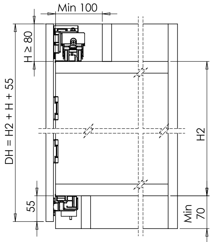
Cabinet without top cover
