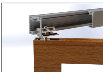
Top Pivot Assembly
