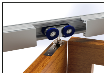
4 wheel intermediate hanger
