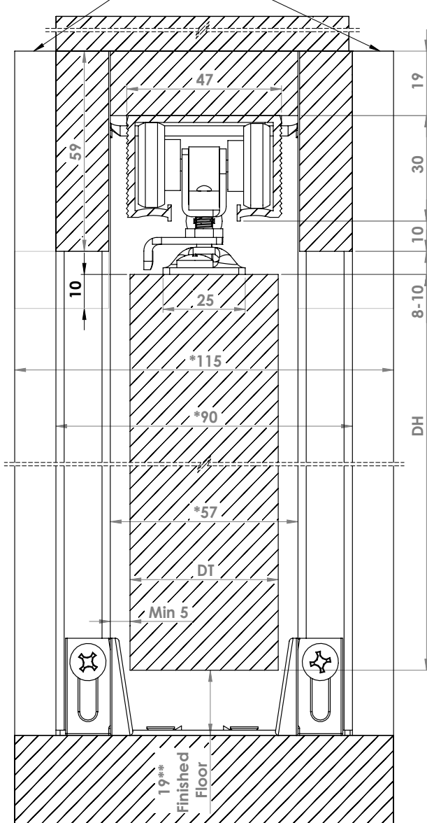
SECTION A-A 12.5mm Plaster Board
